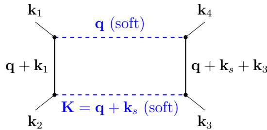
Figure 1: All momentum labels are vectors. Dashed lines select the double-soft region; solid internal lines retain complete hard time dependence.
